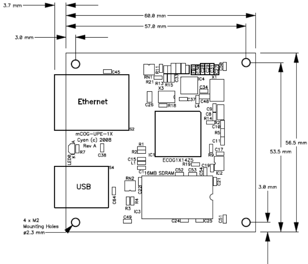
Module outline and mechanical dimensions – top view
