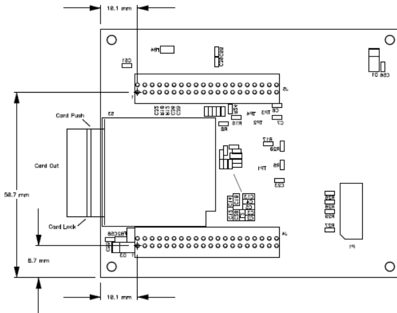
Module connector locations – bottom view
